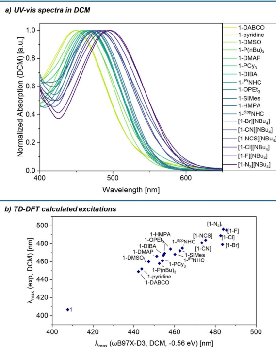
Fig. 6 (a) Normalised CT absorption bands of donor adducts in DCM. (b) Calculated ( \omega B97X-D3/def2-TZVPP/SMD(DCM)// r^2 SCAN-3c) vs. experimentally observed absorption maxima for 1 and donor complexes 1-X/[1-X] − . Calculated absorption wavelengths were redshifted by 0.56 eV.
