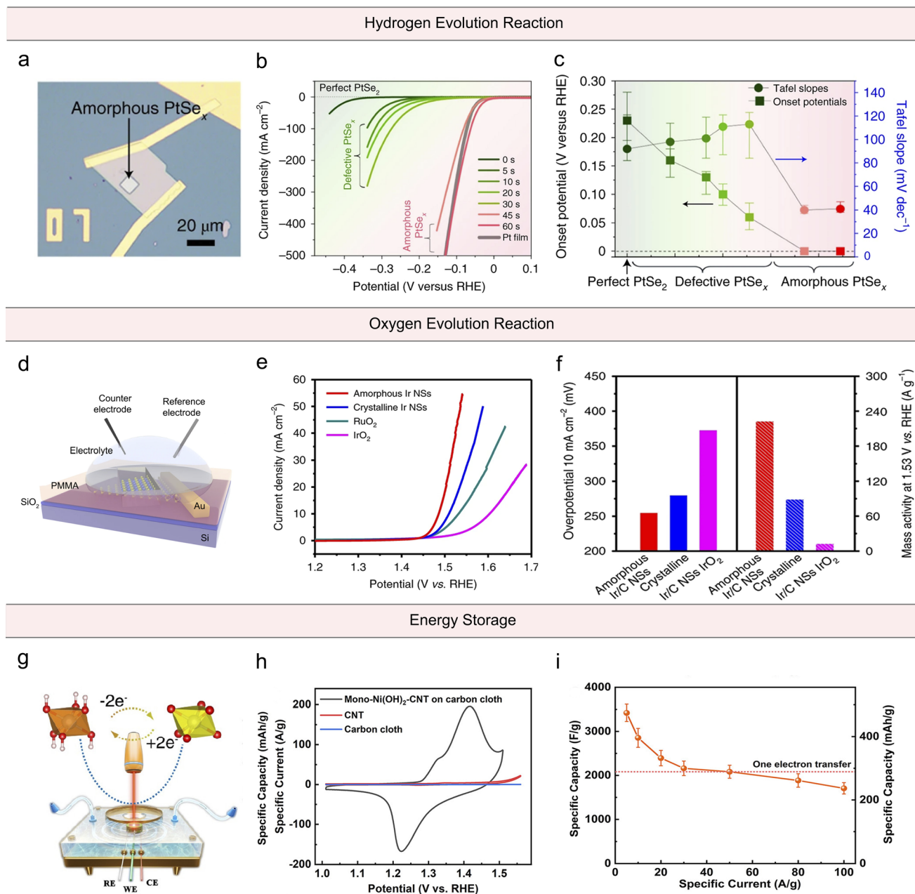
Fig. 10 Electrochemical properties of 2D amorphous materials. (a) Optical micrographs of microelectrochemical cells with single-layer amorphous PtSe x catalysts. (b) HER polarization curves of PtSe x nanosheets. (c) Evolution of HER active sites with Se content: statistical analysis of onset potentials and Tafel slopes across crystalline ( x > 1.5 ), defective ( 1.5 < x < 2 ), and amorphous ( x \leq 1.4 ) phases. Reproduced with permission. 29 Copyright 2022, Springer Nature. (d) On-chip electrochemical microcell (OCEM) configuration for 2D nanocatalyst evaluation: a prepatterned SiO 2 /Si chip with a PMMA-passivated reaction window, immersed in electrolyte with integrated reference/counter electrodes. Reproduced with permission. 86 Copyright 2023 American Chemical. (e) Comparative oxygen evolution reaction (OER) performance of amorphous Ir nanosheets (NSs): polarization curves against crystalline Ir NSs and commercial RuO 2 /IrO 2 benchmarks. (f) Comparison of periplasmic sites and mass activities at 10 \text{ mA cm}^{-2} of amorphous Ir NSs, crystalline Ir NSs, and IrO 2 NSs. Reproduced with permission. 31 Copyright 2019, Springer Nature. (g) In situ Raman spectroscopy setup for monitoring electrochemical phase transitions. (h) Cyclic voltammetry (CV) of single-layer Ni(OH) 2 /CNT composite electrodes, revealing dual redox peaks indicative of Ni 2+ /Ni 4+ transitions. (i) Specific capacity and magnification capability analysis. Reproduced with permission. 47 Copyright 2022 American Chemical Society.
