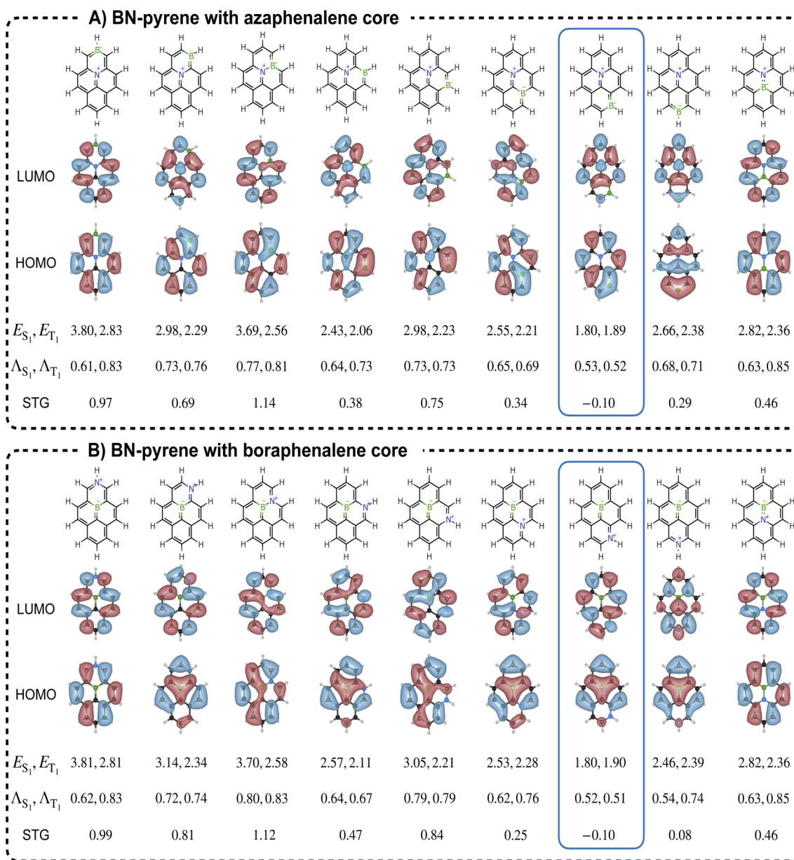
Fig. 4 B,N-substituted pyrenes with azaphenalene (1AP, panel A) and boraphenalene (1BP, panel B) cores: variation in transition energies of the S_1 and T_1 states, and the corresponding STGs predicted with L-CC2/cc-pVDZ. All energies are in eV. Also provided are the \Lambda -indices for S_1 and T_1 transitions, along with the corresponding frontier MOs, calculated at the dh-DFT level.
