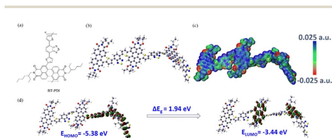
Fig. 31 (a) Molecular structure of BT-PDI polymer; (b) optimized structure of PDI-BT-PDI trimer; (c) MESP of PDI-BT-PDI and (d) frontier molecular structures of PDI-BT-PDI trimer. Reproduced from ref. 174 with permission of RSC.
