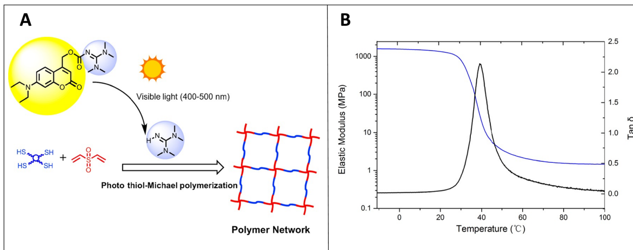
Fig. 11 (A) Base generation from the photobase generator under visible light to initiate the thiol-Michael polymerization. (B) Tan δ and elastic modulus of the thiol-vinyl crosslinked polymeric film made of PETMP and DVS monomers by using 2 wt% coumarin-TMG with 50 mW cm -2 , 400–500 nm irradiation (reproduced from ref. 15 with permission from American Chemical Society, copyright 2016). 15
