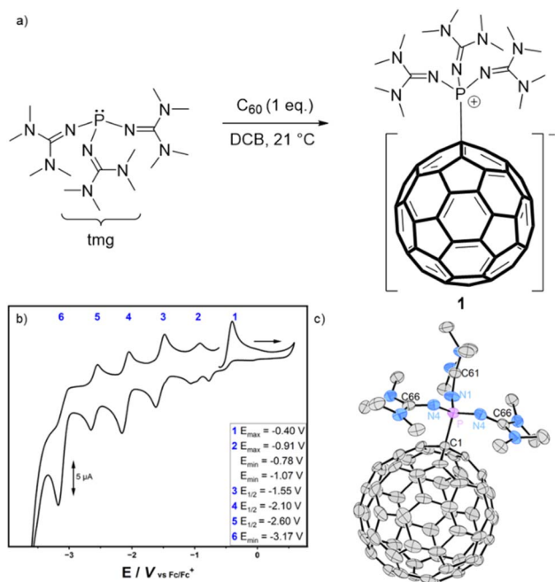
Fig. 2 (a) Reaction of (\text{tmg})_3\text{P} with C_{60} to give 1 ; (b) cyclic voltammogram of 1 in THF at a scan rate of 100 \text{mV s}^{-1} ( \text{Bu}_4\text{NPF}_6 , 0.1 M as electrolyte; Pt working electrode); (c) solid-state structure (positional disorder of C_{60} and THF solvent molecule as well as hydrogen atoms are omitted for clarity); thermal ellipsoids are set at 50% probability, selected bond lengths (Å) and angles (°): P–C1 1.873(2), P–N4 1.6021(16), P–N1 1.606(2), N1–C61 1.304(3), N4–C66 1.308(3), N4–P–N1 117.55(7), N4–P–N4 103.18(12).
