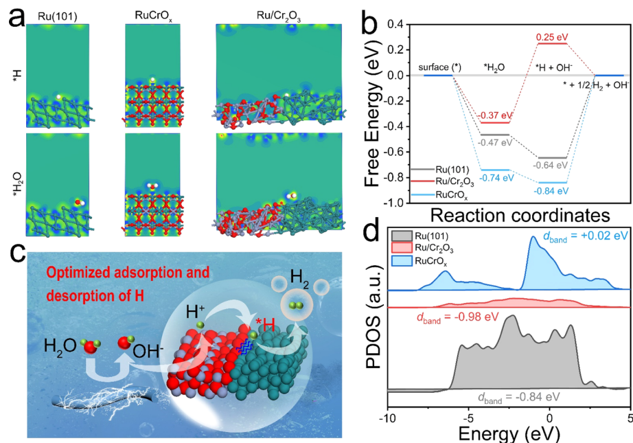
Fig. 5 (a) The charge differential density maps of the adsorption of *H and *H_2O on Ru(101), RuCrO x and Ru/Cr 2 O 3 models, where blue and yellow represent charge electron density decrease and increase, respectively. The green, cyan and red spheres represent Ru, Cr and O atoms, respectively. (b) Calculated adsorption energies of *H_2O and *H on the surface for Ru(101), RuCrO x and Ru/Cr 2 O 3 models. (c) Schematic illustration of the proposed HER catalytic mechanism on Ru/Cr 2 O 3 HNFs. (d) The PDOS of Ru atoms for Ru(101), RuCrO x and Ru/Cr 2 O 3 models.
