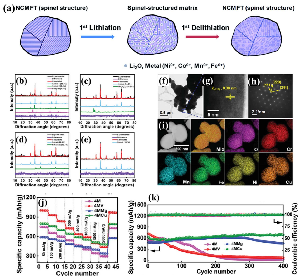
Fig. 10 HESs for LIBs. (a) Charge storage mechanism during initial lithiation and delithiation processes. 109 XRD patterns of (b) (\text{CrNiMnFe})_3\text{O}_4(4\text{M}) , (c) (\text{CrNiMnFeV})_3\text{O}_4(4\text{MV}) , (d) (\text{CrNiMnFeMg})_3\text{O}_4(4\text{MMg}) , and (e) (\text{CrNiMnFeCu})_3\text{O}_4(4\text{MCu}) ; (f) TEM image, (g) high-resolution lattice image, (h) SAED pattern, and (i) HAADF image and EDS mapping of 4MCu; (j) comparative rate capability of various electrodes, and (k) cycling stability of various electrodes at 500 \text{ mA g}^{-1} for 400 cycles. Reproduced with permission. 108 Copyright 2022, John Wiley and Sons.
