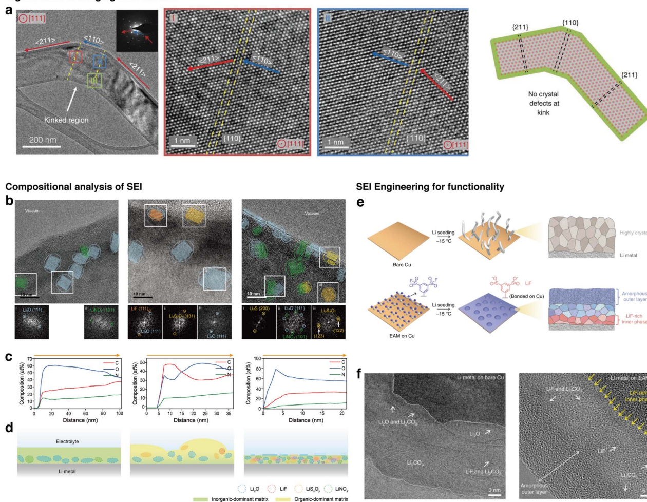
Fig. 2 High-resolution cryo-EM and correlative elemental analysis of battery materials for understanding operation mechanisms. (a) High-resolution imaging of a Li dendrite at the region of a kink, revealing local crystallographic properties of the Li dendrite (reproduced with permission from ref. 26, copyright 2017 AAAS). (b) Images of the SEI revealing areas with local crystallinity, in which the crystallographic phases are determined using fast Fourier transform patterns. (c) Composition profile of C, O, N along the depth of the SEI. (d) Predicted morphologies and composition of the SEI based on cryo-EM analysis (reproduced from ref. 76, copyright 2024 ACS Publications). (e) Scheme for an example of SEI engineering for improving battery performance. (f) Characterization of the SEI for revealing the role of SEI on performance (reproduced from ref. 77, copyright 2020 Nature Publishing Group).
