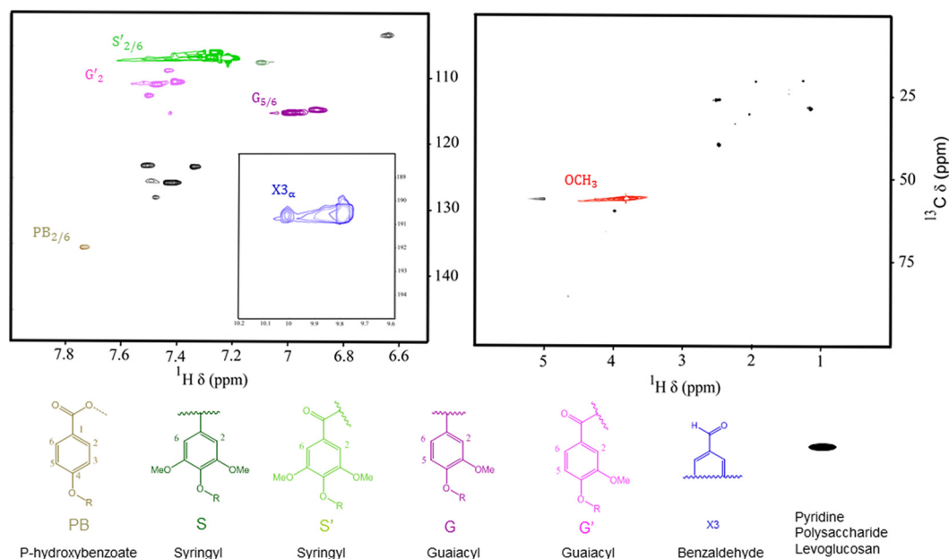
Fig. 15 HSQC NMR spectra of lignin oils obtained under alkaline oxidation conditions. Reaction conditions: 170 ^{\circ}\text{C} , 40 psi oxygen, 19.2 wt% catalyst, 1.25 M NaOH, 32 min.
