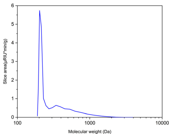
Fig. 14 Molecular weight distribution of lignin oil produced from red oak under oxidation conditions. Reaction conditions: 170 ^{\circ}\text{C} , 40 psi oxygen, 19.2 wt% catalyst, 1.25 M NaOH, 32 min.
