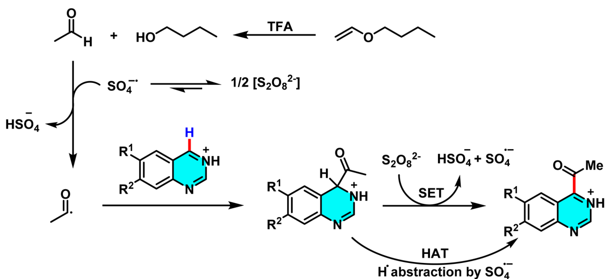
Scheme 83 Plausible reaction mechanism for the acetylation of pyrimidines under metal-free conditions.
