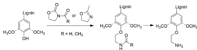
Scheme 16 Lignin amination by two-step amidation-hydrolysis reaction.
