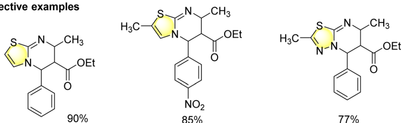
Scheme 41 Synthesis of thiazole using Brønsted acidic ionic liquid Fe 3 O 4 @O 3 Si [PrMIM]HSO 4 .
