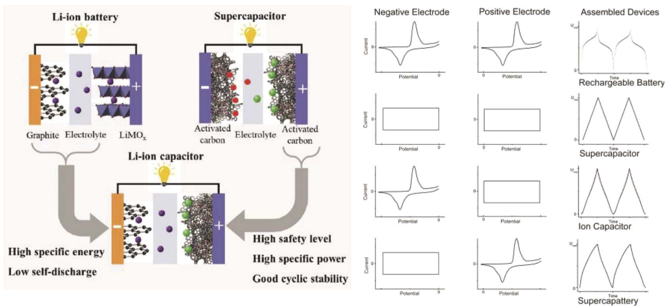
Fig. 13 Li-ion capacitor (LIC) utilizes the best features of super capacitors with the benefits of Li-ion batteries by combining materials developed by IFE ( https://www.ife.no/en/from-wood-chips-and-silicon-to-high-power/ ) and comparison of CV and charge–discharge profile of different types of energy storage devices. 121 [Reproduced from ref. 121 with permission from The Royal Society of Chemistry, copyright 2025].
