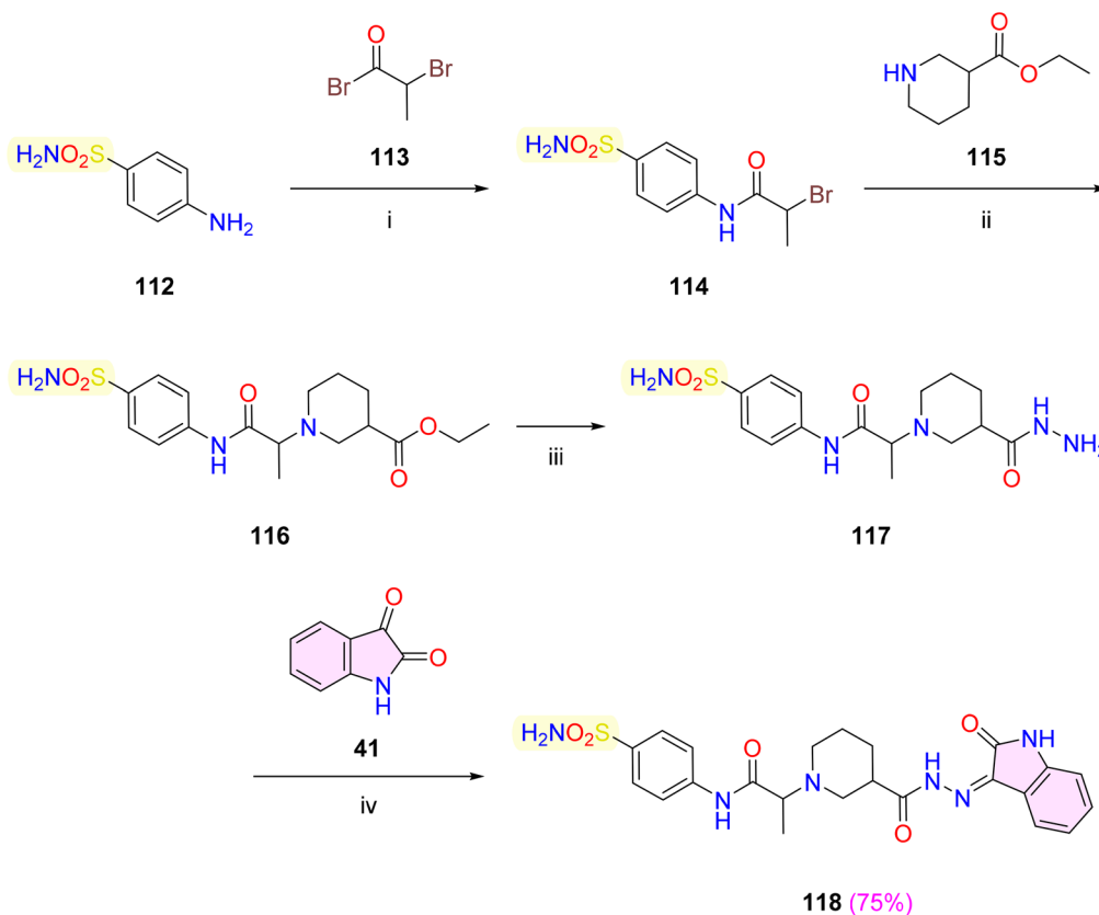
Scheme 19 Synthesis of isatin-sulphonamide hybrid 118 . Reagents and conditions: (i) dioxane, \text{Et}_3\text{N} , stirring, r.t., 20 h; (ii) acetone, \text{K}_2\text{CO}_3 , KI, stirring, r.t., 2 h; (iii) \text{N}_2\text{H}_4 \cdot \text{H}_2\text{O} , EtOH, reflux, 4 h; (iv) EtOH, gl. AcOH (cat.), reflux, 6 h.
