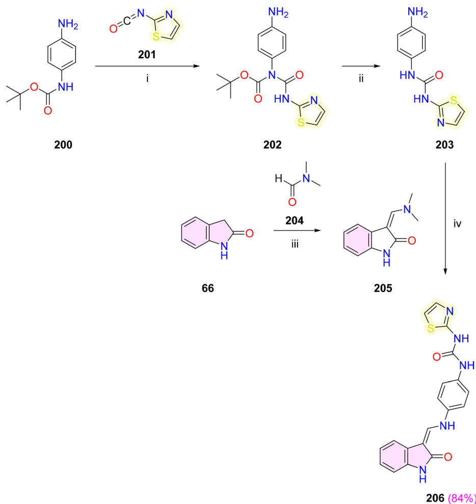
Scheme 39 Synthesis of isatin-thiazole hybrid 206 . Reagents and conditions: (i) DCM, -25 \text{ }^{\circ}\text{C} to r.t.; (ii) TFA, DCM, 0 \text{ }^{\circ}\text{C} ; (iii) toluene, reflux, 2 h; (iv) AcOH, reflux, 4 h.
