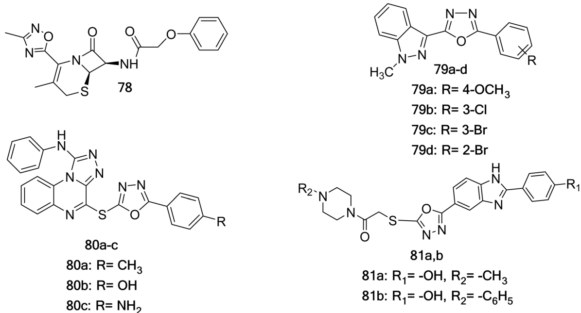
Fig. 14 Compounds (78–81).
