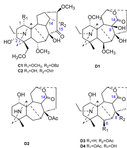
Fig. 5 Structures of pyro- and lactone-type C 19 -DAs.
