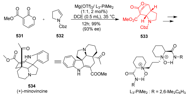
Scheme 69 IEDDA reaction of 2-pyrones 531 with enamine 532 in total synthesis of (+)-minovincine ( 534 ). 138
