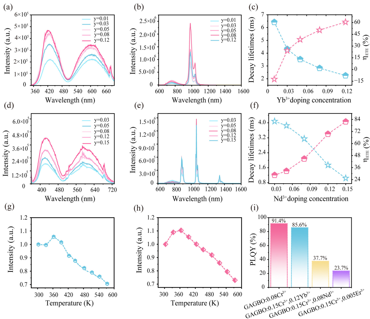
Fig. 4 The (a) excitation spectra and (b) emission spectra of GAGBO:0.15Cr 3+ ,yYb 3+ ( y = 0.01 – 0.12 ). (c) Decay lifetimes and energy transfer efficiency ( \eta_{\text{ETE}} ) dependent on the Yb 3+ doping concentration. The (d) excitation spectra and (e) emission spectra of GAGBO:0.15Cr 3+ ,yNd 3+ ( y = 0.03 – 0.15 ). (f) Decay lifetimes and \eta_{\text{ETE}} dependent on the Nd 3+ doping concentration. The normalized integrated emission intensity diagram of (g) GAGBO:0.15Cr 3+ ,0.12Yb 3+ and (h) GAGBO:0.15Cr 3+ ,0.08Nd 3+ . (i) PLQY measurement of GAGBO:0.15Cr 3+ ,0.12Yb 3+ and GAGBO:0.15Cr 3+ ,0.08Nd 3+ .
