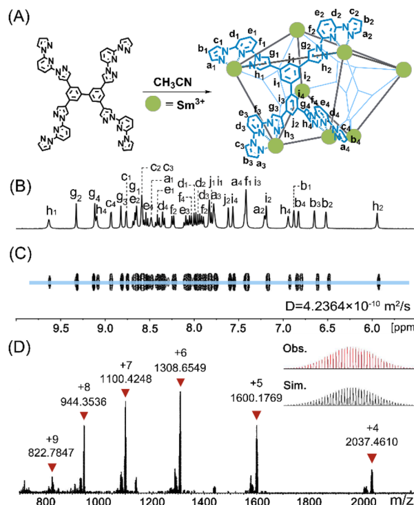
Fig. 2 (A) Self-assembly of \text{L} with \text{Sm}(\text{OTf})_3 . (B) ^1\text{H} NMR spectra (400 MHz, 298 K) of \text{Sm}_8\text{L}_4 in \text{CD}_3\text{CN} . (C) DOSY spectra of \text{Sm}_8\text{L}_4 . (D) ESI-TOF-MS of \text{Sm}_8\text{L}_4 with the inset showing the observed and simulated isotopic patterns of the +6 peak.
