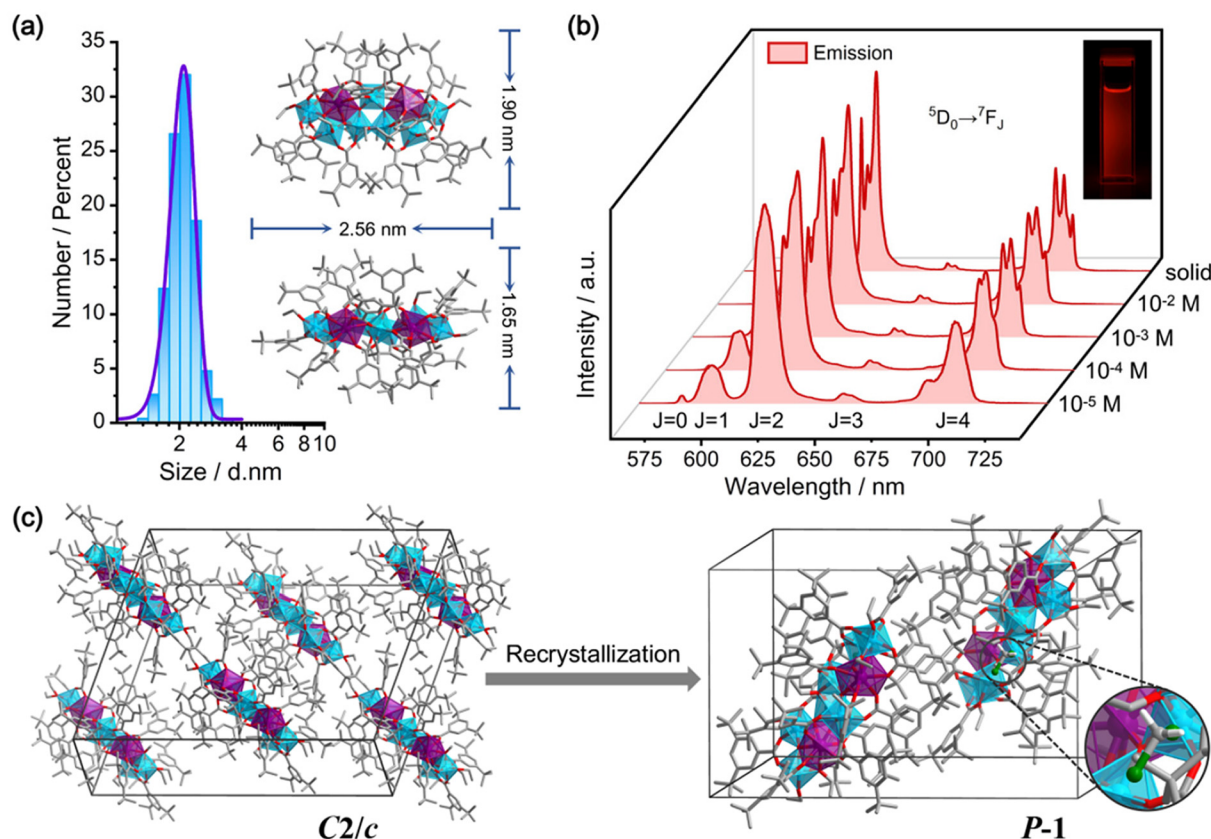
Fig. 3 (a) Dynamic light scattering analysis of \text{Eu}_2\text{Ti}_7 . (b) Emission spectra of \text{Eu}_2\text{Ti}_7 solutions at various concentrations. (c) The space group transition from C2/c to P\bar{1} after recrystallization of \text{Eu}_2\text{Ti}_7 .
