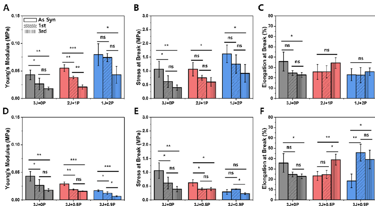
Fig. 8 Tensile measurements of on-stoichiometry cases (A–C) and off-stoichiometry excess amine cases (D–F) for three reprocessing cycles. Data are presented as the mean ± standard deviation ( n = 3-5 ). The statistical analysis was conducted using a multiple group comparison through one-way analysis of variance along with Tukey's post hoc test. "ns" = not-significant, * = p -value < 0.05, ** = p -value < 0.01, *** = p -value < 0.001.
