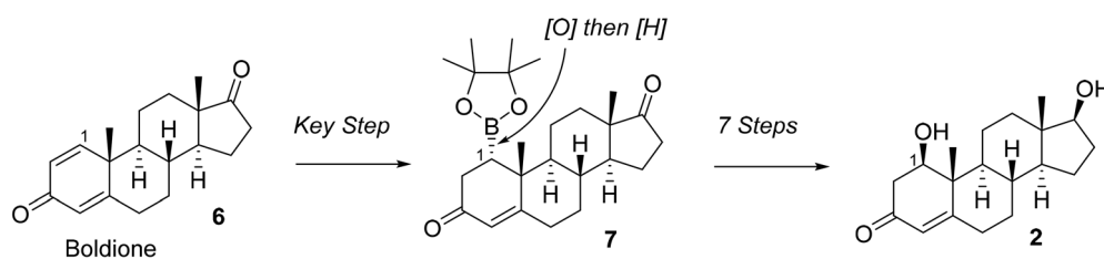
Fig. 2 Overall strategy in this report to synthesize 1 \beta -hydroxytestosterone (2) from boldione (androst-1,4-dien-3,17-dione, 6) through a boronated intermediate (7).
