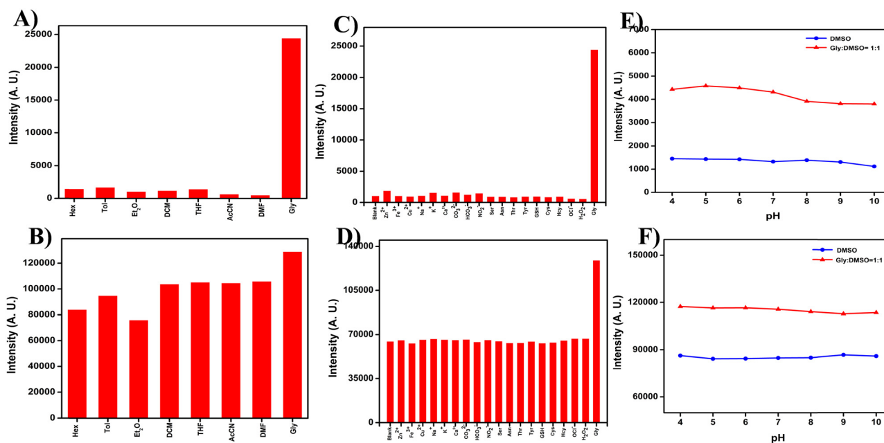
Fig. 2 Emission studies of compounds (A) 7 and (B) 8 in different solvent polarity. Emission spectra of compounds (C) 7 and (D) 8 in DMSO with various competitive species (100 \mu\text{M} ) (blank, Zn(OAc) 2 , FeCl 3 , Cu(OAc) 2 , NaCl, KCl, CaCl 2 , K 2 CO 3 , NaHCO 3 , NaNO 2 , Ser, Asn, Thr, Tyr, GSH, Cys, Hcy, OCl - , H 2 O 2 , and glycerol). Emission studies of compounds (E) 7 and (F) 8 at different pH values and viscous media (DMSO and DMSO : glycerol = 1 : 1) (2 \mu\text{M} , \lambda_{\text{ex}} = 350 nm).
