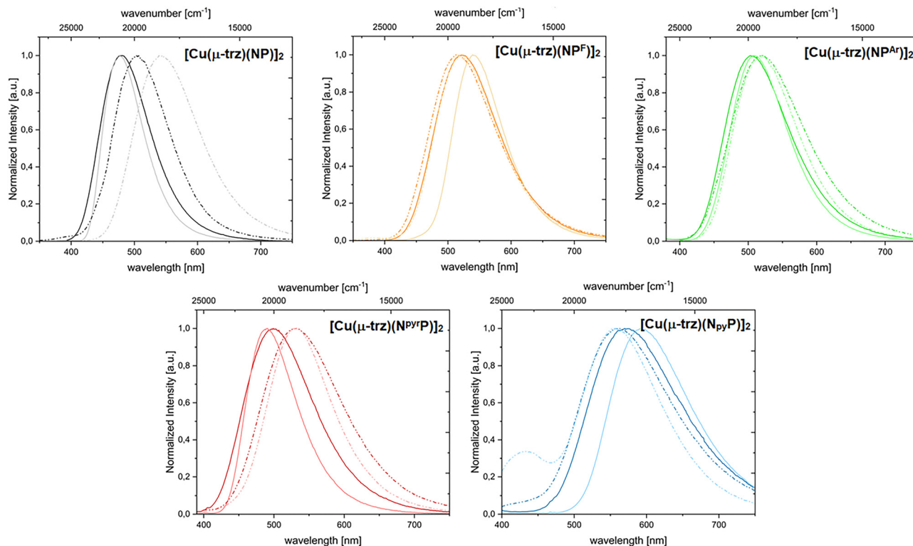
Fig. 4 Emission spectra of [\text{Cu}(\mu\text{-trz})(\text{NP})]_2 (black), [\text{Cu}(\mu\text{-trz})(\text{NPF})]_2 (orange), [\text{Cu}(\mu\text{-trz})(\text{NPA})]_2 (green), [\text{Cu}(\mu\text{-trz})(\text{NPyP})]_2 (red) and [\text{Cu}(\mu\text{-trz})(\text{NpyP})]_2 (blue) in the solid state (solid lines) and PMMA matrix (dashed lines). Vivid and faded colours refer to the data collected at 297 K and 77 K respectively.
