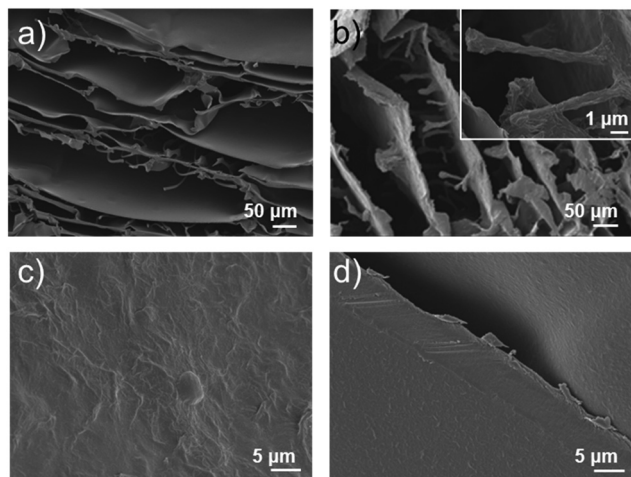
Fig. 2 Morphology of the foams. SEM cross-sectional images of an alginate (a) and 5%Ti 3 C 2 T x -alginate foam; inset shows details at higher magnification (b). Images of the foam wall surfaces of 5%Ti 3 C 2 T x -alginate and alginate foams (c), (d).
