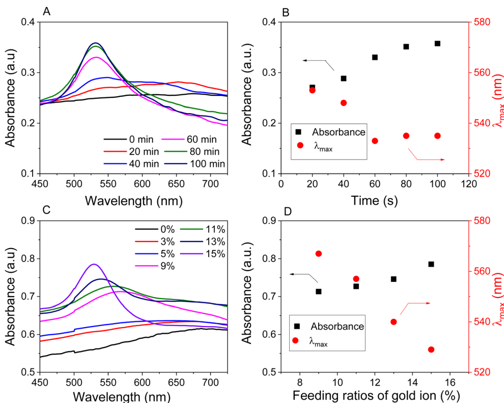
Fig. 2 UV-vis spectra (left) and plots of absorbance and wavelength (right) as functions of reaction conditions: reaction time for the sample with a feeding gold ion ratio of 15% (A and B), and various feeding ratios of gold ion to nanocomposite (w/w) (C and D).
