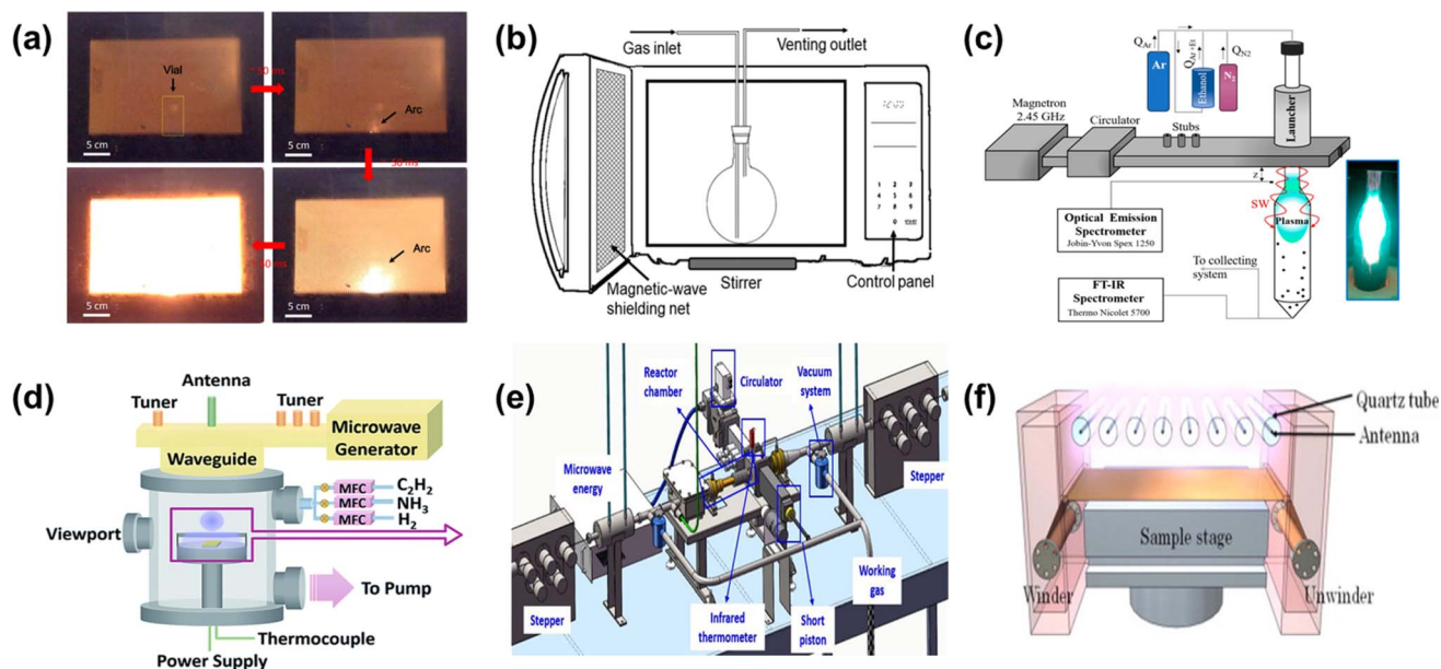
Fig. 4 Schematic diagram of various types of microwave reactors. (a) The domestic microwave oven. (b) Adapted domestic microwave oven. (c) Typical composition diagram of an MPCVD reactor. (d) MPCVD for large area reaction zone type. (e) Continuous microwave plasma reactor systems for the production of fibres. (f) Systems of a roll-to-roll microwave plasma reactor.
