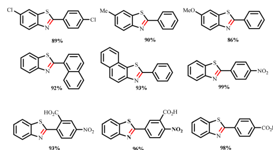
Scheme 37 Reaction between 2-aminobenzenethiol and benzonitrile catalyzed by an \text{Fe}_3\text{O}_4@SiO_2\text{-bis(aminopyridine)-Cu(II)} nanocomposite (Mahmood et al. ).
