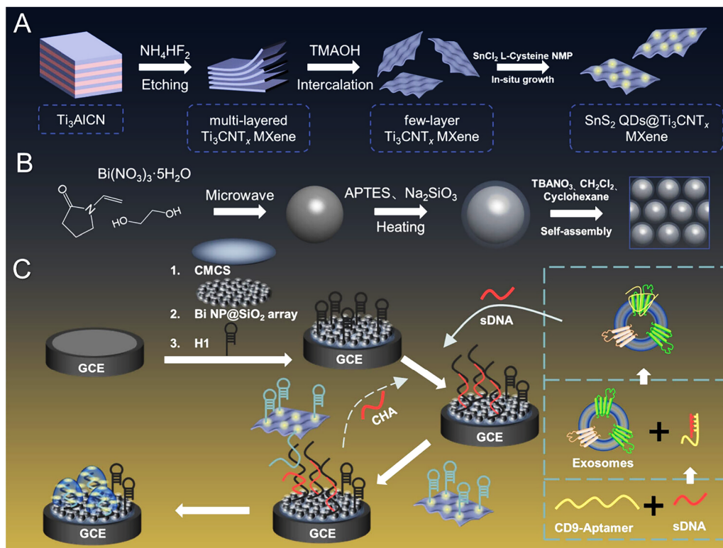
Fig. 7 This illustration showcases the ECL sensing system that incorporates \text{SnS}_2 quantum dots@MXene Ohmic junctions and a \text{Bi@SiO}_2 nanoparticle array, crucial for the detection of CD9-exosomes. The first step (A) involves creating the \text{SnS}_2 QDs@MXene heterojunction, where the quantum dots are synthesized to enhance electrochemiluminescence. This combination forms a robust junction that reduces contact resistance, thereby improving charge injection efficiency. Following this, the \text{Bi@SiO}_2 nanoparticle array is assembled (B), designed to optimize surface plasmon resonance. The arrangement of Bi nanoparticles within the \text{SiO}_2 matrix is essential for maximizing the interaction with the emitted ECL from the \text{SnS}_2 QDs@MXene junction. Finally, the sensing process for CD9-exosome detection occurs when the ECL interacts with the \text{Bi@SiO}_2 array (C), leading to amplified luminescence and enabling sensitive identification of these exosomes in saliva. Carboxymethyl chitosan (CMCS), catalyzing hairpin self-assembly (CHA), (3-aminopropyl)triethoxysilane (APTES), carboxymethyl chitosan (CMCS). Reproduced with permission from ref. 67 Copyright 2024 American Chemical Society.
