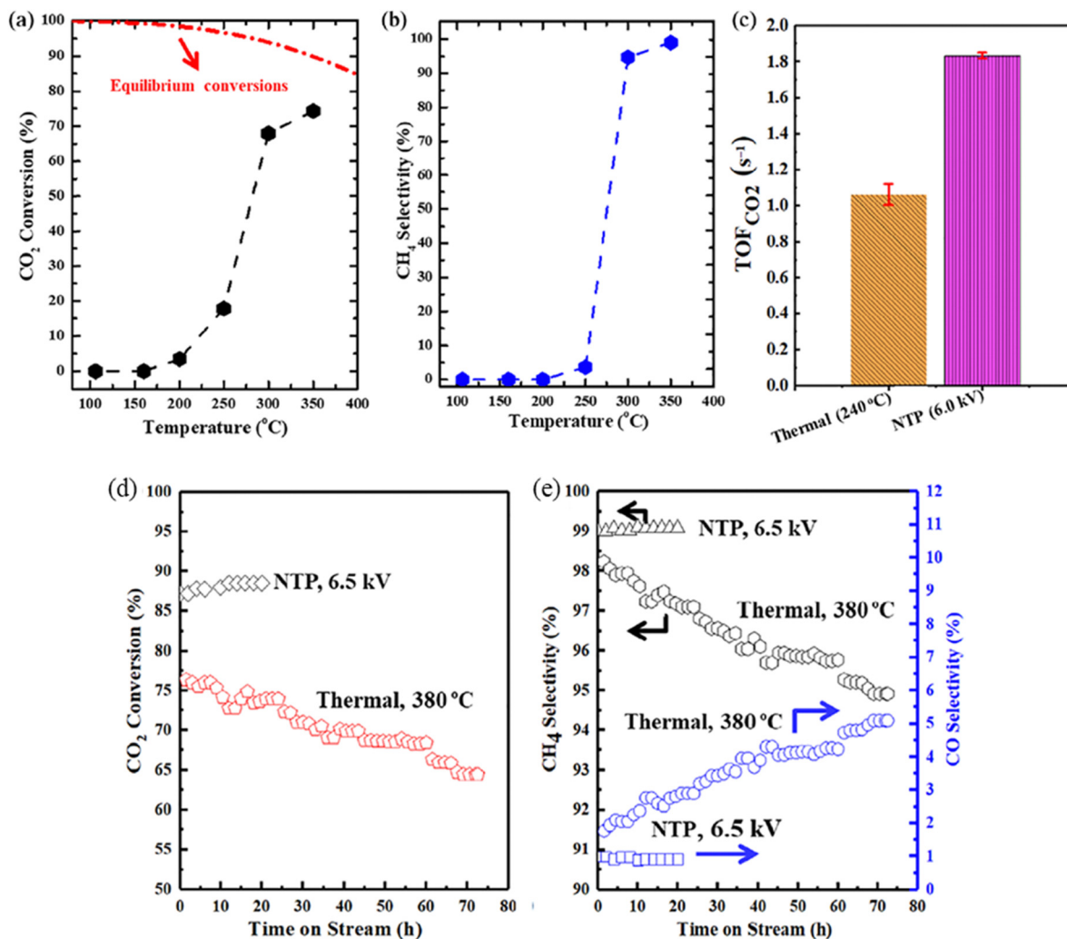
Fig. 11 Performance comparison of catalytic hydrogenation of \text{CO}_2 over the 15Ni/UiO-66 catalyst with thermal and NTP activation: (a) conversion of \text{CO}_2 and (b) selectivity of \text{CH}_4 for thermal activation, and (c) TOF amount of \text{CO}_2 conversion. The as-synthesized catalyst stability study for catalytic hydrogenation of \text{CO}_2 by thermal ( 380^\circ\text{C} ) and NTP (6.5 kV) activation: (d) conversion of \text{CO}_2 , (e) selectivity of CO and \text{CH}_4 . Reproduced from ref. 100 with permission from John Wiley and Sons, copyright 2019.
