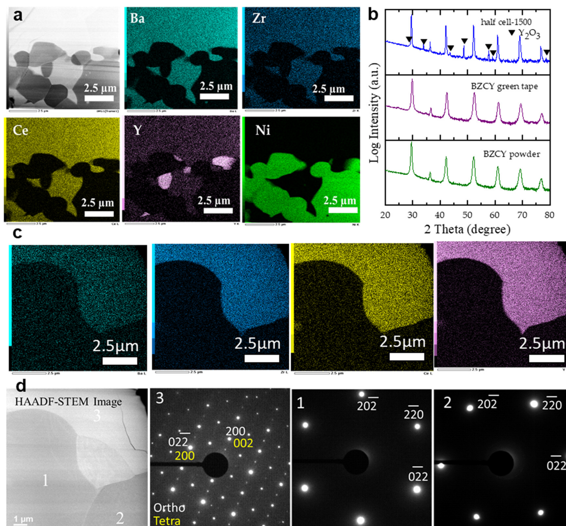
Fig. 3 (a) HAADF micrograph of a cross-sectional lamella of BZCY44362|NiO-BZCY44362 electrode interface with corresponding EDS maps of Ba, Zr, Ce, Y, Ni. (b) Room-temperature X-ray diffraction patterns of BZCY44362 powder, green tape, and the half-cell after sintering at 1500 ^{\circ}\text{C} . (c) HAADF micrograph of the BZCY44362|NiO-SZCY541 interface with corresponding EDS maps of Ba, Zr, Ce, Y (d) selected-area electron diffraction pattern with Miller indices and labeled crystallographic direction for Ni and SZCY541.
