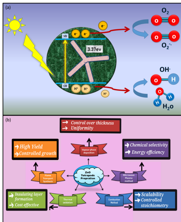
Fig. 6 (a) Photocatalytic mechanism of ZnO TPs (b) schematic (a) displaying various strategies for the synthesis of ZnO TPs along with their useful characteristics.
