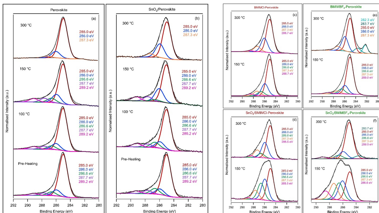
Fig. 2 High-resolution C 1s core level XPS spectra of the pure ((a) and (b)) and IL-modified ((c)–(f)) perovskite films deposited on Ti foil ((a), (c) and (e)) and SnO 2 coated Ti foil ((b), (d) and (f)). Peak intensities are normalised to the intensity of the adventitious carbon peak. BEs of fitted peaks are shown next to each spectrum and a summary of C 1s peak assignments is shown in Fig. 1.
