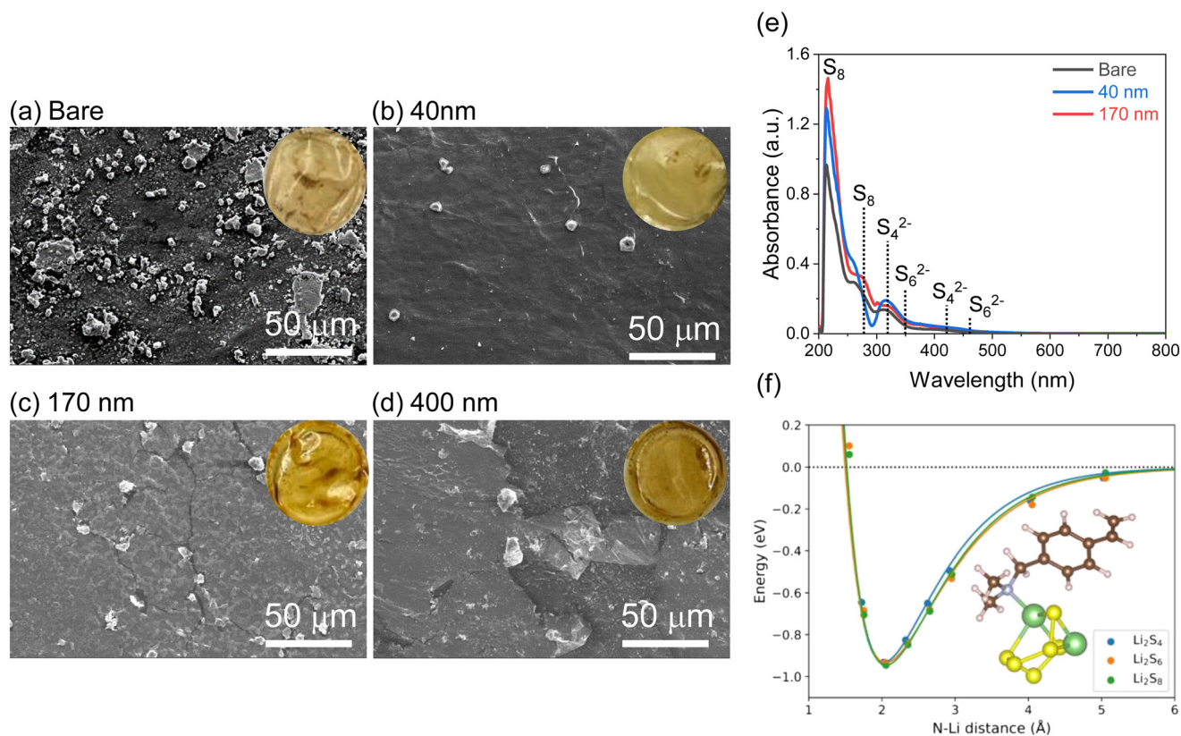
Fig. 8 (a–d) Scanning electron micrographs of bare, 40 nm-, 170 nm-, and 400 nm-iCVD@PE separators after 20 charge-discharge cycles. Inset: optical images of recovered separators. (e) UV-vis spectra of solutions used to extract the respective harvested separators. (f) Binding energy of \text{Li}_2\text{S}_n to a DMAMS monomer, plotted as a function of N-Li distance. Points represent DFT data, and lines are fits to a Morse potential. Inset: visualization of the bonded DMAMS monomer and \text{Li}_2\text{S}_6 molecule (H shown in gray, C in brown, N in blue, Li in green, and S in yellow).
