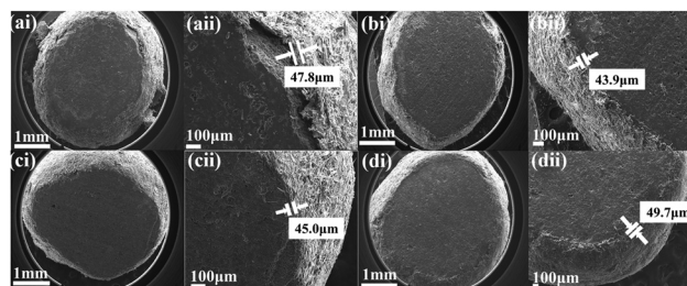
Fig. 4 Cross-sectional SEM images showing the average thickness of (ai), (aii) feather microfibril coated with urea as a control coating (KC), and (bi), (bii); (ci), (cii); and (di), (dii) three different feather microfibril zinc-coated urea samples with 3%, 6%, and 9% coating content (KZC1, KZC2, and KZC3), respectively.
