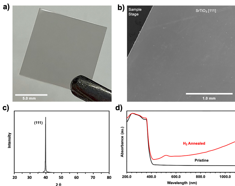
Fig. 2 (a) Photo of (111) \text{SrTiO}_3 single crystal, as purchased. (b) SEM image of \text{SrTiO}_3 single crystal surface after \text{H}_2 annealing. (c) XRD Pattern of \text{H}_2 annealed \text{SrTiO}_{3-x} single crystal, confirming the (111) orientation (d) Optical absorbance spectra before and after \text{H}_2 annealing.
