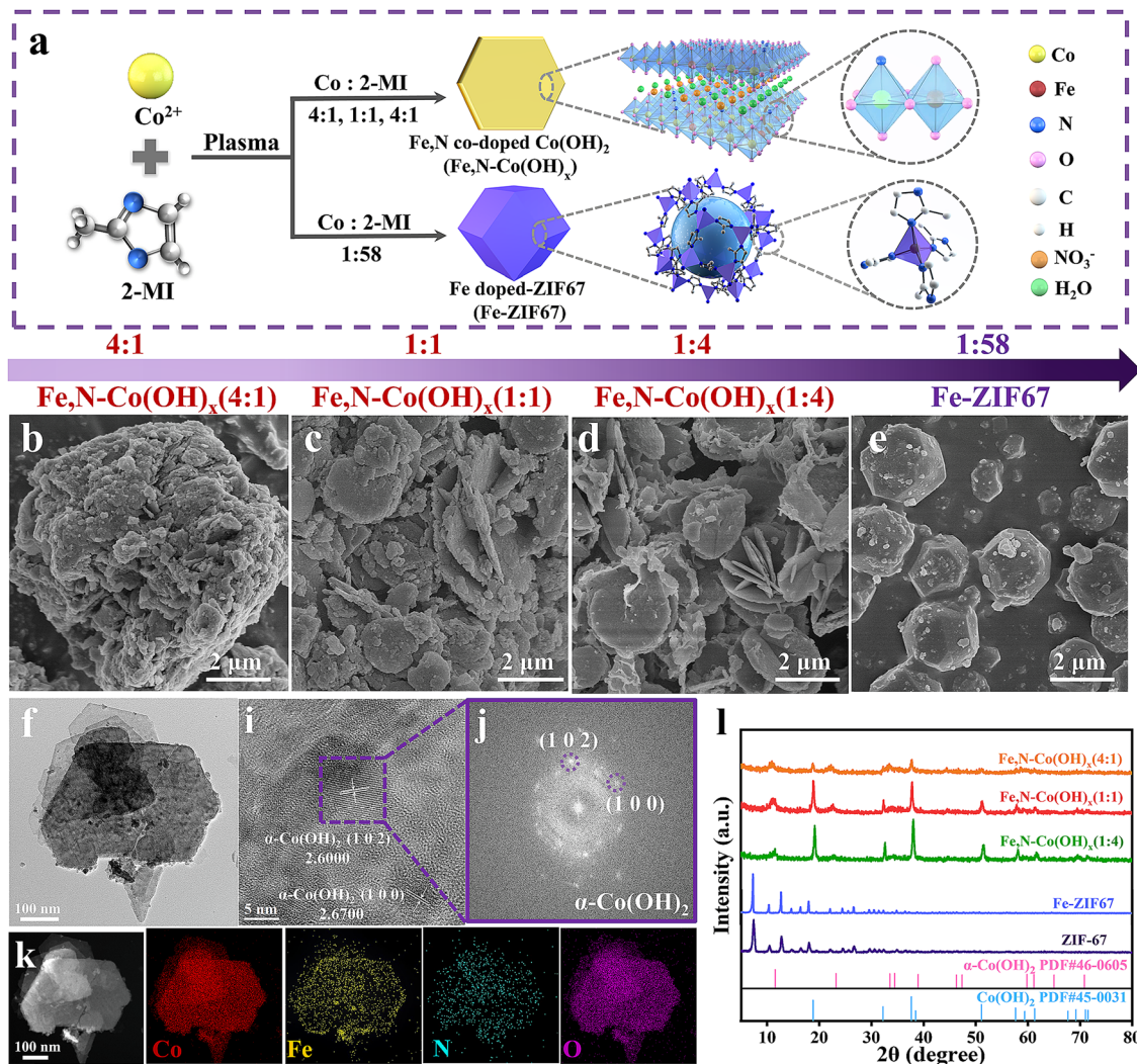
Fig. 1 Preparation process and morphology of electrocatalysts. (a) Schematic of the synthesis of Fe,N co-doped Co(OH) 2 ( i.e. , Fe,N-Co(OH) x ) and Fe-doped ZIF67 ( i.e. , Fe-ZIF67) induced by plasma in water. (b)–(e) SEM images of (b) Fe,N-Co(OH) x (4 : 1), (c) Fe,N-Co(OH) x (1 : 1), (d) Fe,N-Co(OH) x (1 : 4), and (e) Fe-ZIF67. (f)–(k) Morphology and elemental distribution of Fe,N-Co(OH) x (1 : 1): (f) TEM images, (g) HAADF-STEM images, (h) corresponding FFT pattern, and (i) EDS mapping images. (l) XRD patterns of Fe,N-Co(OH) x (4 : 1) (orange line), Fe,N-Co(OH) x (1 : 1) (red line), Fe,N-Co(OH) x (1 : 4) (green line), and Fe-ZIF67 (purple line).
