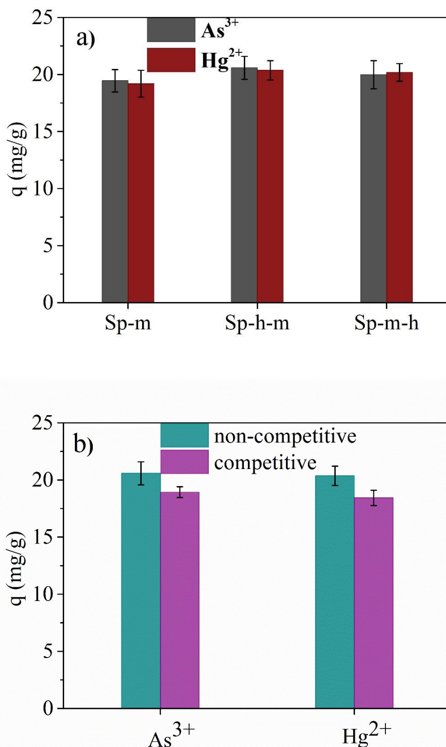
Figure 6. a) The adsorbed quantities of \text{As}^{3+} and \text{Hg}^{2+} in mg/g of Sp-m, Sp-h-m and Sp-m-h sponges in the experiments of single metal ion solutions and b) the adsorbed \text{As}^{3+} and \text{Hg}^{2+} on the Sp-h-m sponge in the experiment of the competitive adsorption.
