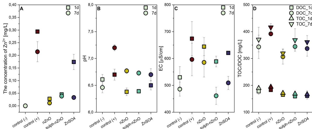
Fig. 3 Zn 2+ concentrations (A), pH (B), EC (C), and DOC and TOC (D) in the growth medium of barley following exposure to Zn compounds for 1 and 7 days. The control (-) and the control (+) mean the untreated plants grown in HGL solutions without or with Zn ions (as ZnSO 4 ), respectively. Error bars represent standard error ( n = 3 repeats).
