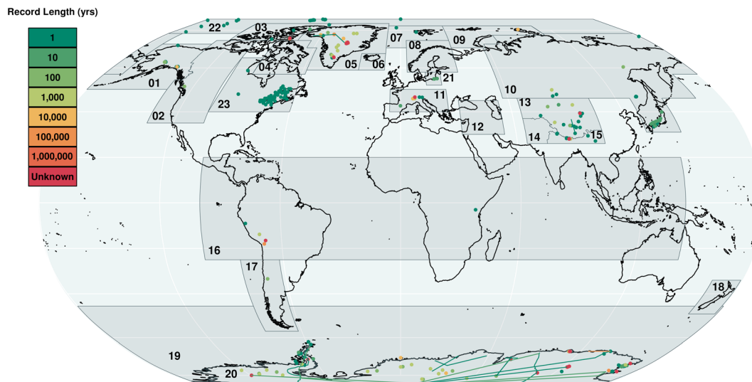
Fig. 3 The Robinson map projection shows the global records of Pb concentration and isotopes from Tables A.1 and A.2. † Sampling sites for Pb work in snow and ice are colored by temporal length. When samples were collected as a traverse, the path is illustrated as a solid line as the best approximation. Note: some traverse lines have artifacts due to incomplete trip logistical data. For ease of discussion, the Pb records are broken into 23 regions, the 20 first-order regions from the Global Terrestrial Network for Glaciers, 64 plus three author-defined regions. These regions are mapped on the figure with grey boxes, labeled with their numerical glaciated region code ( i.e. , 01 for Alaska). See Table 1 for a complete list of glacier region names and codes. To see how these sample sites compare to the known glaciers mapped in the Randolph Glacier Inventory, 65 see ESI figure. † 20
