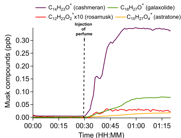
Fig. 2 The time series of musk compounds following the injection of 10 \mu\text{l} of perfume into the 8 m 3 smog chamber was measured by the Vocus. Cashmeran, galaxolide, astratone, and rosamusk were identified in the commercial perfume. We used the sensitivity of cashmeran at m/z 207.1743 (4115 cps ppb -1 ) to convert the Vocus signals of galaxolide m/z 259.2056, astratone ( m/z 271.1904), and rosamusk ( m/z 199.1693) into mixing ratios. Note that the concentration of rosamusk was multiplied by a factor of 10 for scaling.
