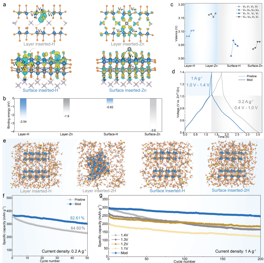
Fig. 4 Theoretical calculations and molecular dynamic simulation. (a) Electron density differences of NVO after layer and surface insertion of H^+ and Zn^{2+} , respectively. (b) Binding energy for ion insertions. (c) The valence state of vanadium atoms around the insertion site. (d) Galvanostatic and modified charge-discharge curves of Zn/NVO batteries. (e) MD simulation results of all types of proton insertion conditions in 2 M ZnSO_4 electrolytes. Cycling performance of batteries with different cut-off voltage and modification at 0.2 A g^{-1} (f) and 1 A g^{-1} (g), respectively.
