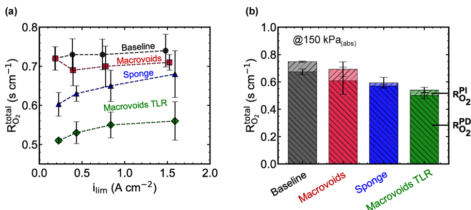
Fig. 5 Comparing oxygen mass transport resistances between GDMs (a) total oxygen mass transport resistance ( R_{O_2}^{total} ) as measured at four different O 2 concentrations (1, 2, 4 and 8%) by the oxygen limiting current method first proposed by Baker et al. 42 measured at 100% relative humidity. (b) Breakdown of R_{O_2}^{total} into the pressure dependent ( R_{O_2}^{PD} ) and pressure independent ( R_{O_2}^{PI} ) oxygen mass transport resistance at 2% O 2 in N 2 at 150 kPa abs for all different GDMs.
