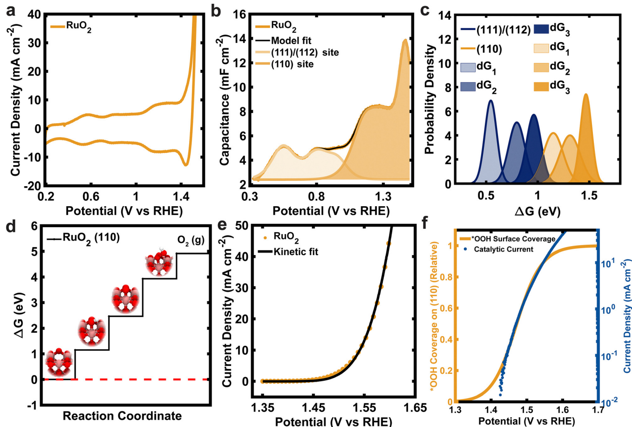
Fig. 2 Electrodesorption and kinetic analysis of RuO 2 electrocatalyst synthesized at 700 °C. (a) Cyclic voltammogram scanned at 1 V s -1 . (b) Comparison of electroadsorption model fits of (111)/(112) and (110) sites to electroadsorption profile derived from (a). (c) Distributions of reaction energies for the first three electron-transfer steps involved in the OER. (d) Free energy diagram constructed from electroadsorption analysis. (e) Comparison between steady-state current density and kinetic model fit. (f) Surface coverage of *OOH species on (110) site and catalytic current density versus potential.
