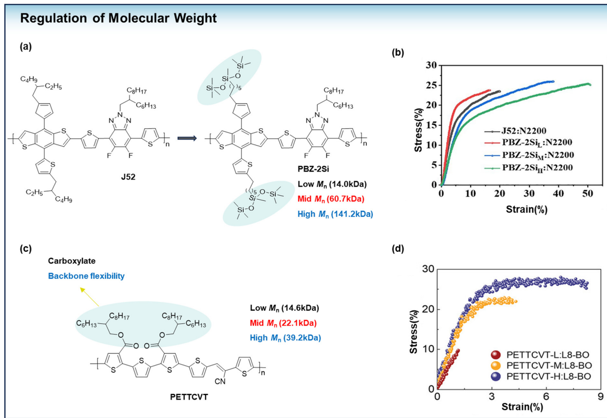
Fig. 2 (a) The chemical structure of PBZ-2Si L , PBZ-2Si M and PBZ-2Si H . (b) The stress-strain curves of the J52/PBZ-2Si L /PBZ-2Si M /PBZ-2Si H :N2200 blend films under the pseudo free-standing tensile test. (c) The chemical structure of PETTCVT. (d) The stress-strain curves of the PETTCVT-L/PETTCVT-M/PETTCVT-H:L8-BO. (a) and (b) Reproduced with permission from ref. 32. Copyright 2022, Elsevier. (c) and (d) Reproduced with permission from ref. 33. Copyright 2023, Wiley-VC.
