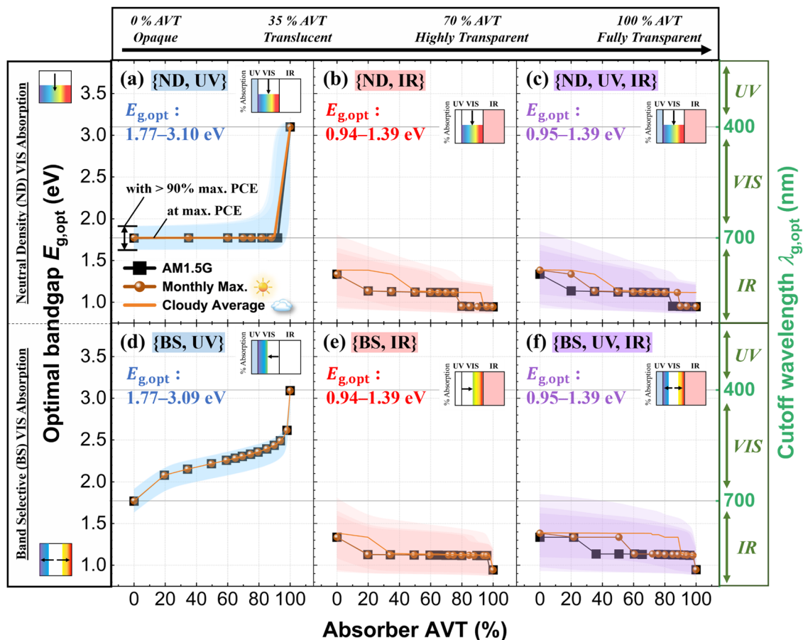
Fig. 9 The PCE-optimal bandgap ( E_{g,opt} ) vs. AVT over the three irradiance conditions (AM1.5G, monthly max. and cloudy avg.) for the neutral density (ND, top row, a–c) and band selective (BS, bottom row, d–f) methods and the UV (left column, a and d), IR (middle column, b and e), and UV + IR (right column, c and f) absorption modes. The lines refer to the bandgap for the max. PCE. The shaded regions correspond to the range of bandgaps where the limiting PCE reaches over 90% of the maximum value. Regions of deeper colours as the overlap of those corresponding to various irradiance conditions indicates higher confidence levels. A wider bandwidth characterizes a higher tolerance of bandgaps for optimal STPV performance.
