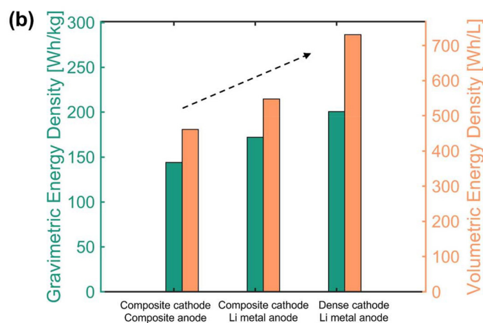
Fig. 1 (a) Schematic illustration of SSBs consisting of a composite anode and a composite cathode, a Li metal anode and a composite cathode, and a Li metal anode and a crystallographically oriented dense cathode. (b) Theoretical gravimetric and volumetric energy densities for each of these SSB designs (anode/separator/cathode basis).
