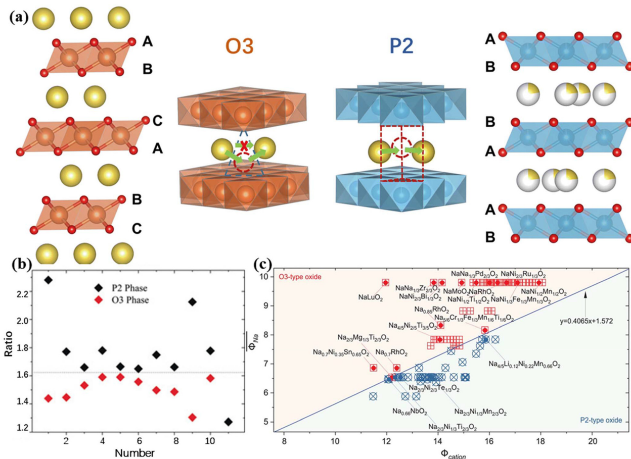
Fig. 2 Crystal structures of the O3 and P2 phases and predictive methodologies for their identification. (a) Crystalline structure of layered oxide cathode materials and the \text{Na}^+ migration path. 57 Copyright 2024, Royal Society of Chemistry. (b) The ratio of the interlayer distance between the alkali metal layer d_{(\text{O}-\text{Na}-\text{O})} and the transition metal layer d_{(\text{O}-\text{TM}-\text{O})} . 58 Copyright 2018, Wiley-VCH GmbH. (c) Various sodium based LTMOS with the O3 and P2 structures, which show clear tendency toward each structure depending on the sodium ionic potential and the overall cationic potential. 59 Copyright 2020, The American Association for the Advancement of Science.
