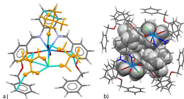
Fig. 4 (a) Capped stick representation of [\text{TMA}][1\text{-Cl}] , surrounded by neighboring cations. Cations are shown in orange. Cyan lines represent short intermolecular contacts below the sum of the van der Waals radii of the respective atoms. Hydrogen atoms involved in short contact interactions are represented as isotropic spheres; (b) mixed capped stick/spacefill view of one of the tetrameric [[\text{TMA}][1\text{-Cl}]_4] units representative of the packing elements in the structure. Color chart: grey = C, white = H, blue = N, red = O, green = Cl, and light blue = U.
